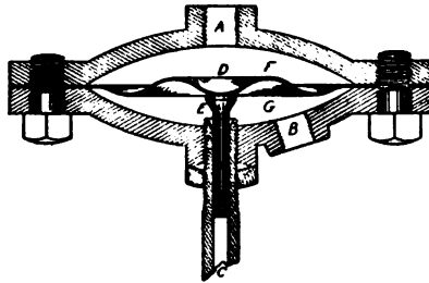
FIG. 910.—Gasoline Burner Regulator, operating with a corrugated diaphragm, like a steam gauge. A is the inlet for steam; B, the inlet for liquid gasoline; C, the port leading to the burner; D, the diaphragm; E, the head on the grooved rod of the valve; F, the steam chamber; G, the gasoline chamber.
